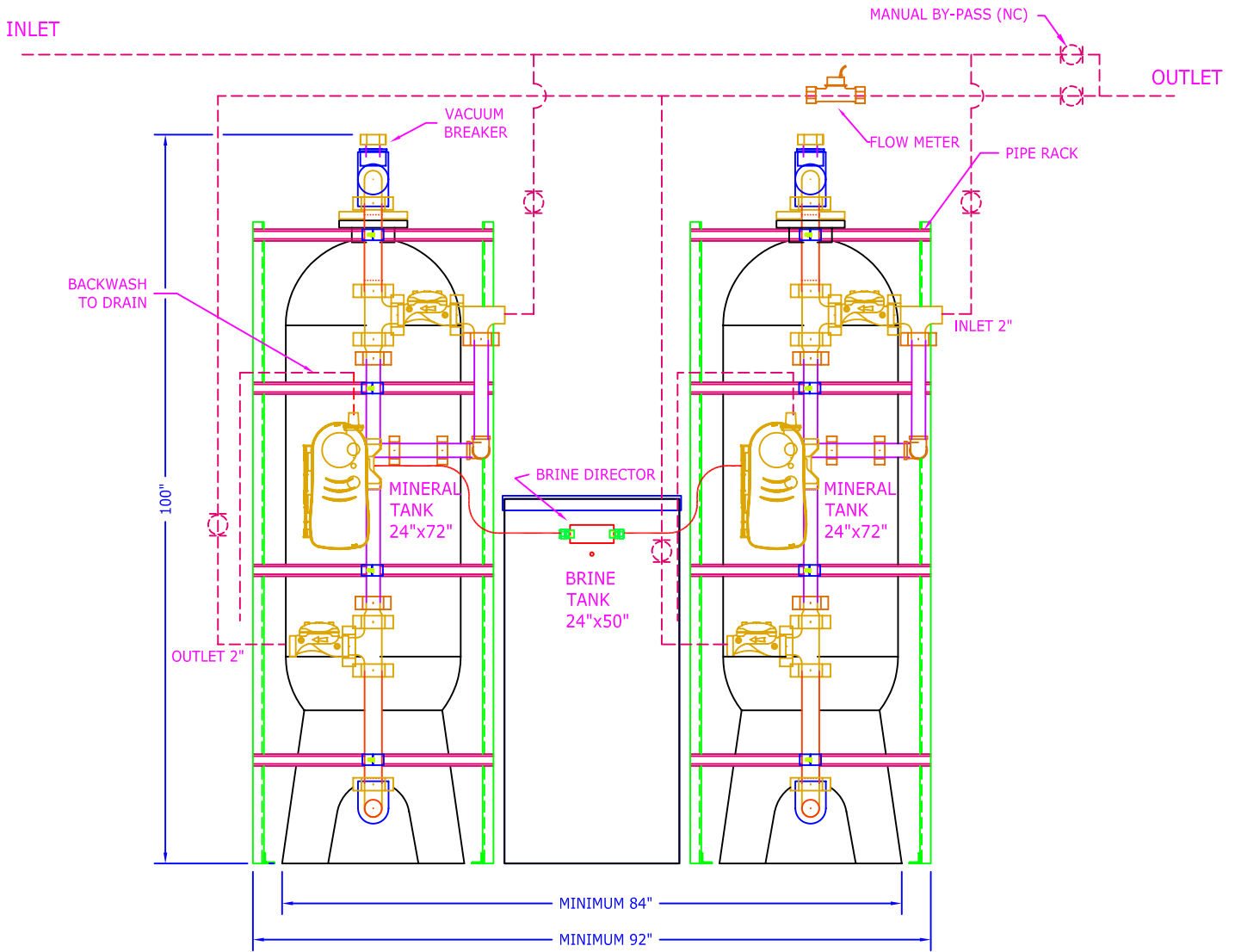
FRONT VIEW
