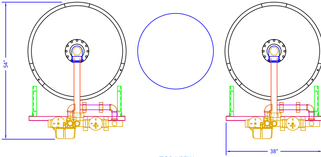
TOP VIEW
