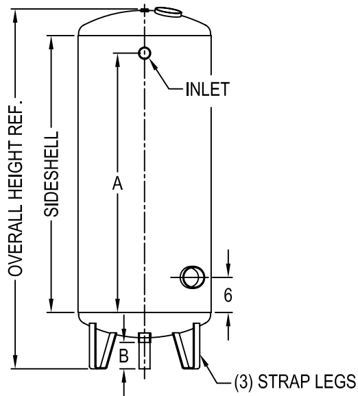
DIMENSIONAL CHART
