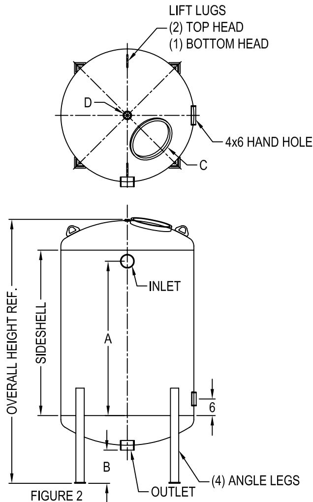
DIMENSIONAL CHART
