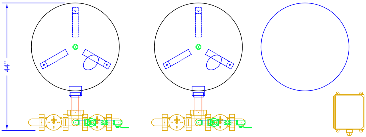
TOP VIEW
