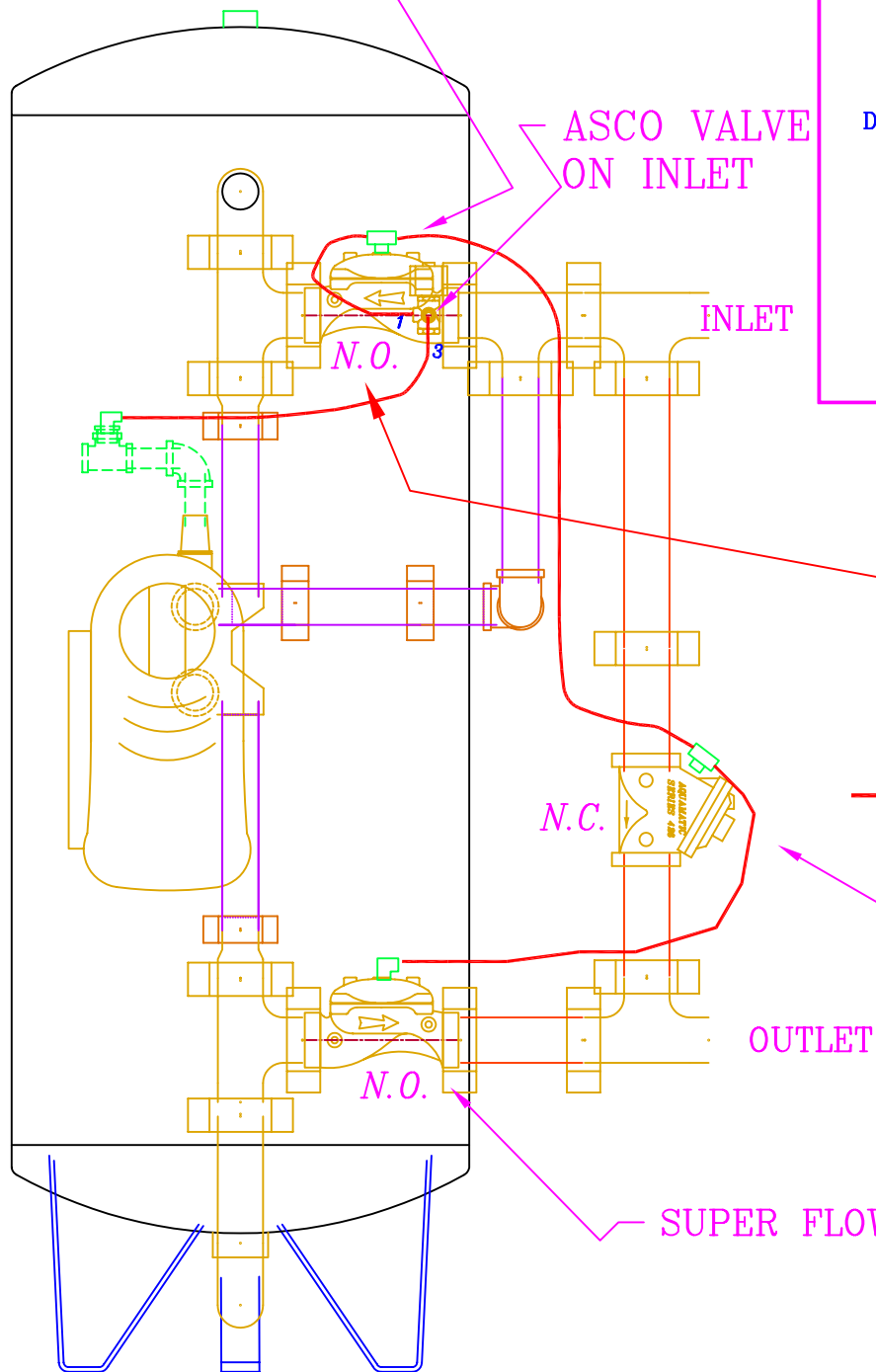
INLET VALVE DETAIL
